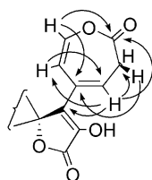
Figure 4. Selected HMBC relationships for the oxepinone moiety of retipolide C ( 7 ).
