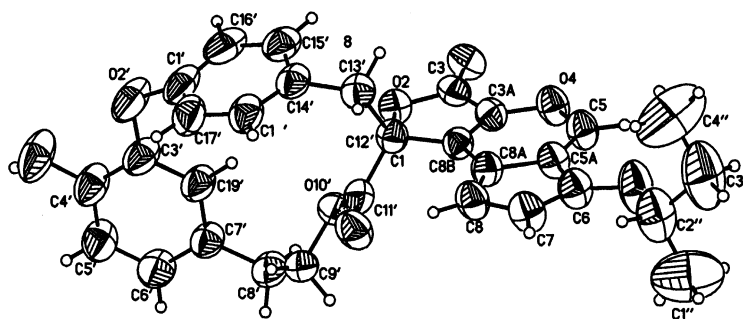
Figure 3. ORTEP plot derived from a single-crystal X-ray analysis of anhydretipolide A 6- O -( S )- sec -butyl ether ( 2b ).
