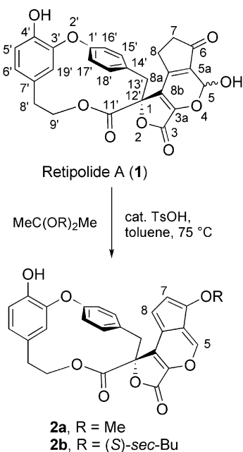
Scheme 2. Conversion of retipolide A into anhydretipolide A 6- O -alkyl ethers 2 .
