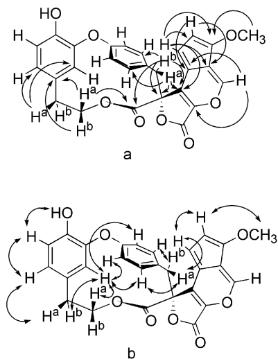
Figure 2. Selected HMBC (a) and NOE (b) relationships for anhydretipolide A 6- O -methyl ether ( 2a ).
