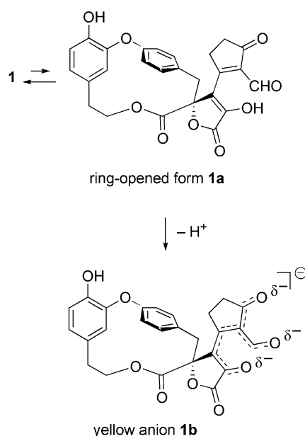
Scheme 3. Formation of the delocalized yellow anion 1b from retipolide A ( 1 ).
