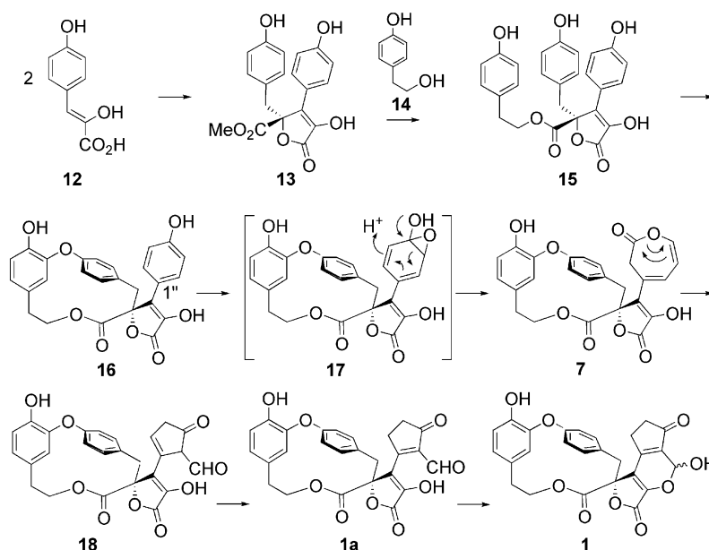
Scheme 4. Proposal for the biosynthesis of butyrolactone II ( 13 ), secoretipolide E ( 15 ), retipolide E ( 16 ), retipolide C ( 7 ), and retipolide A ( 1 ).
